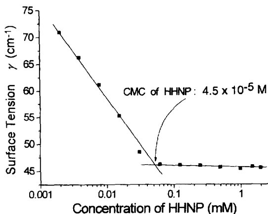
Figure 1. Surface tension ( \gamma ) vs. [HHNP]. See text for conditions.
