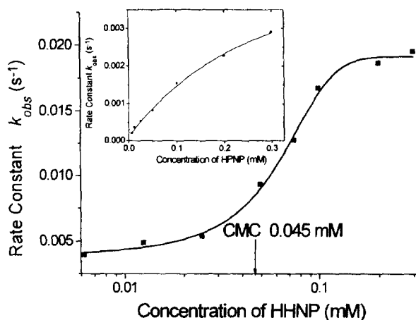
Figure 2. k_{\text{obs}} , \text{s}^{-1} , for the \text{Eu}^{3+} -mediated cleavage of HHNP as a function of [HHNP]. 11 Inset: An analogous plot for HPNP.
